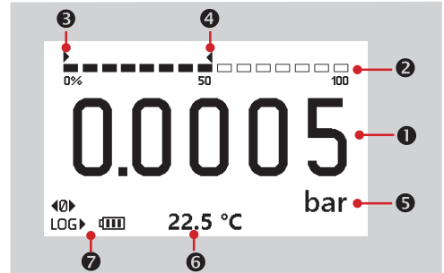
Figure 6.1: elements of the measuring mode
