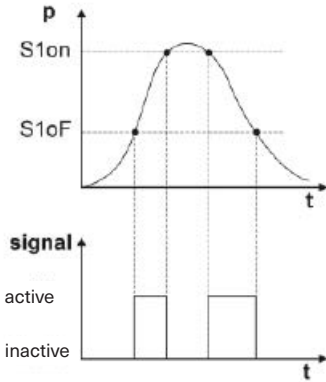
Figure 4: comparison mode inverted
