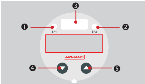
Figure 2: keypad for devices with 2 switching outputs
