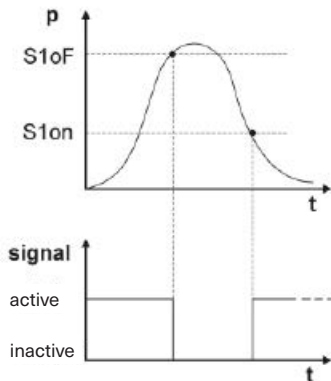
Figure 6: hysteresis mode inverted
